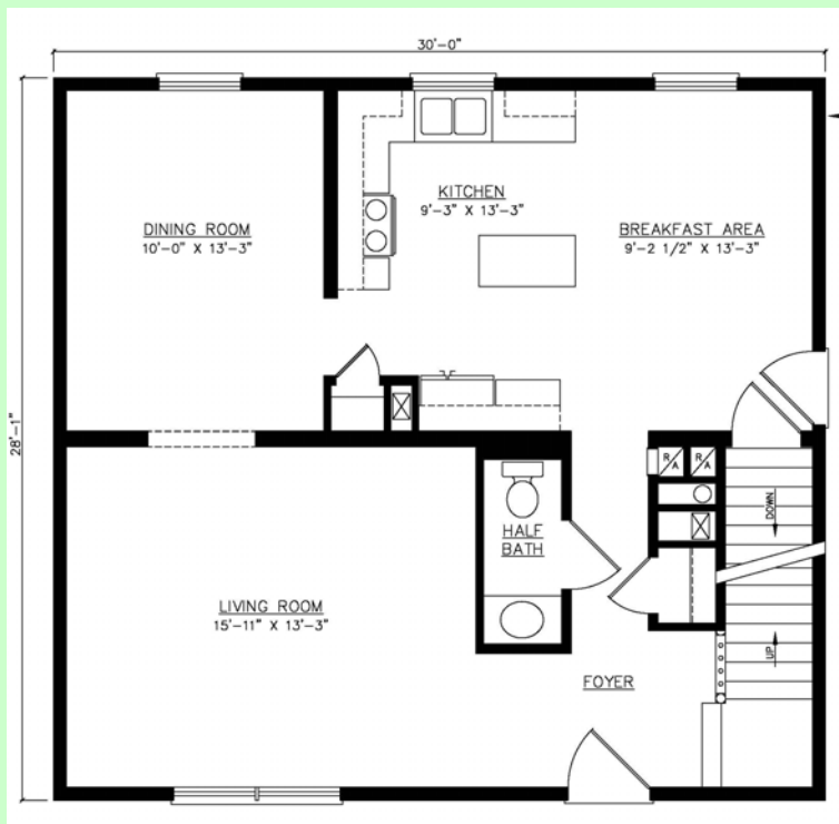
1st Floor Basement Plan
