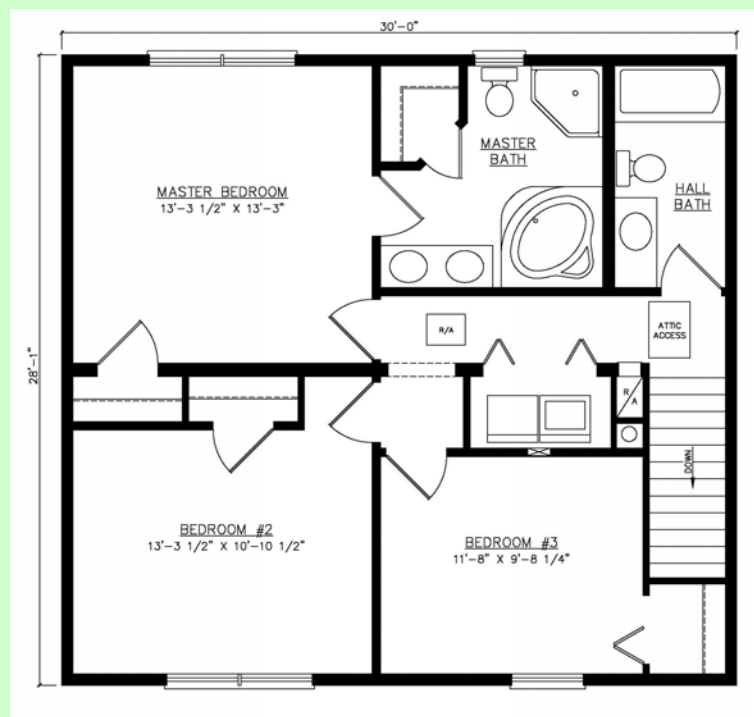
2nd Floor
