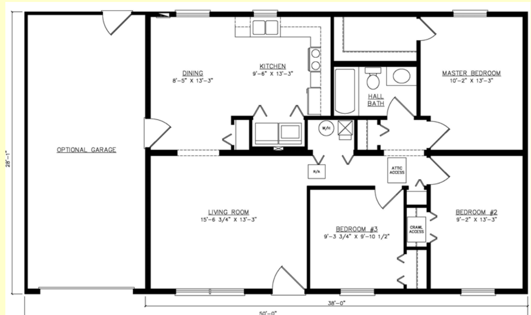
Crawlspace Plan
