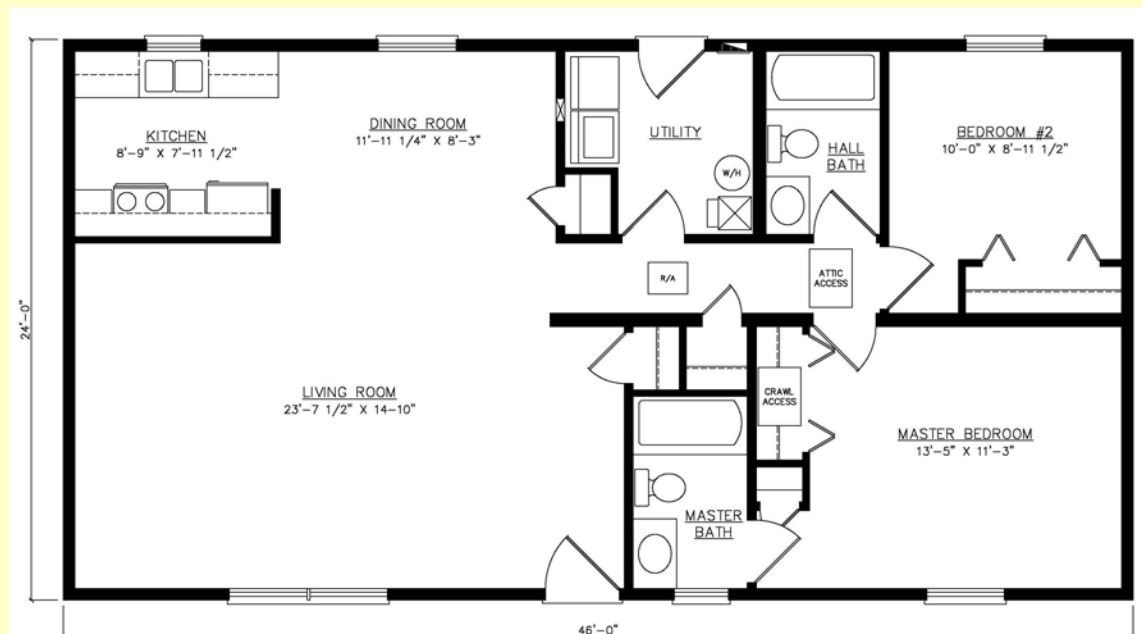
Crawlspace Plan
