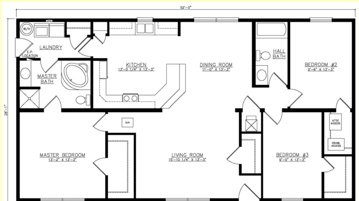
Crawlspace Plan
