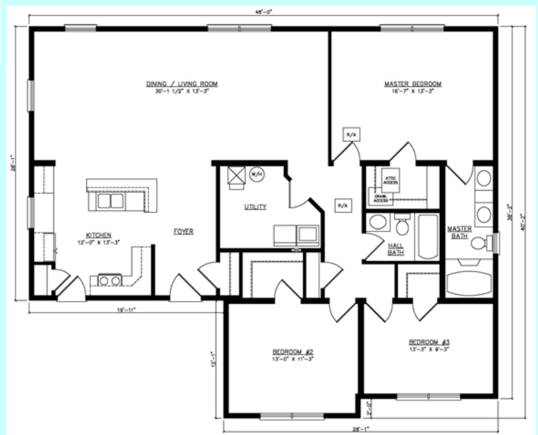
Crawlspace Plan
