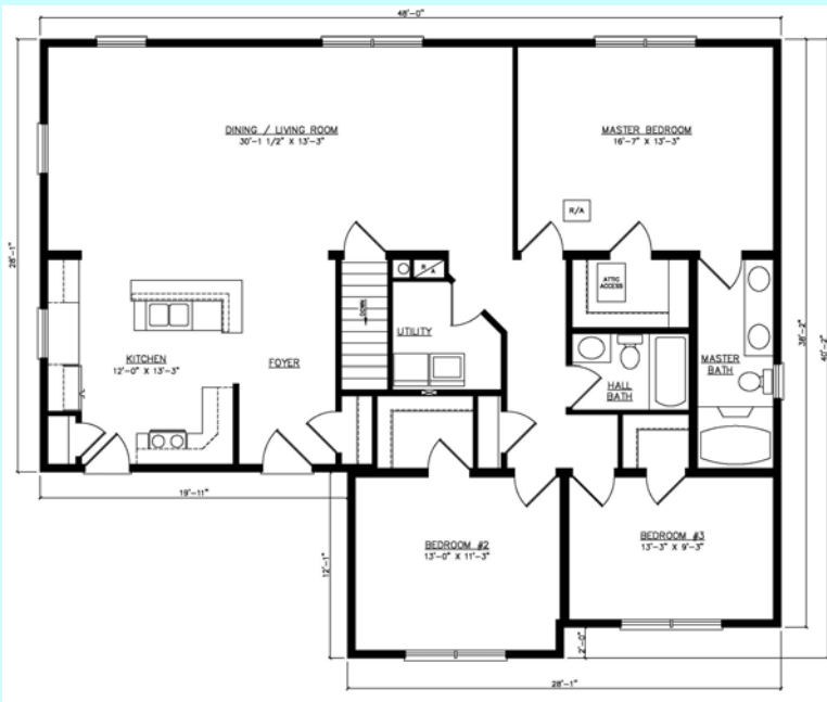
Basement Plan
