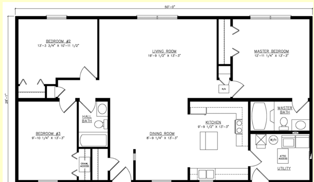
Crawlspace Plan
